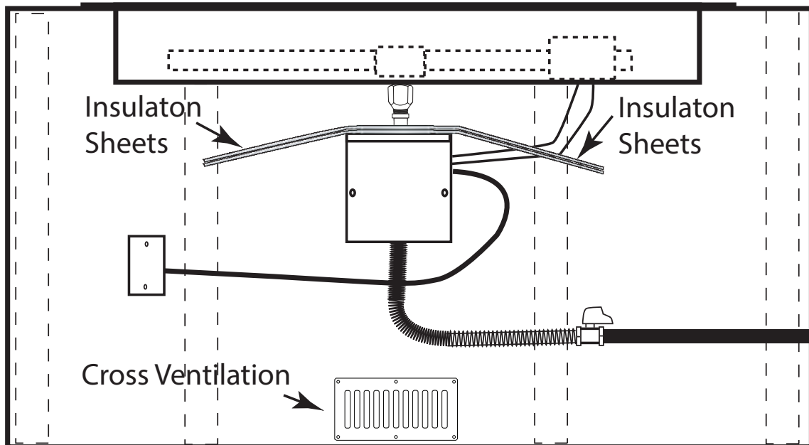
Fig. 2 Insulation installed over top of stainless steel box.
