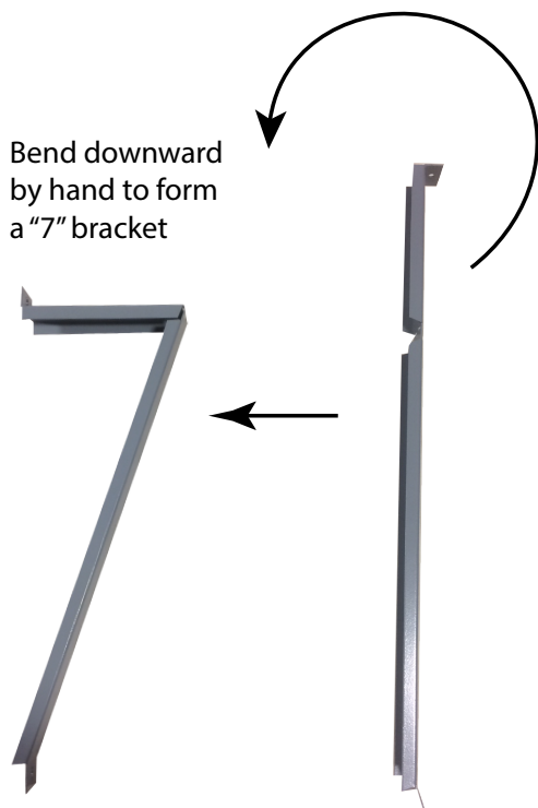
Fig. 1 Bending the "7" Bracket
